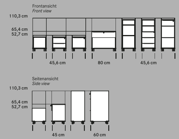
WINEA MAXX Caddy WINEA MAXX caddy
