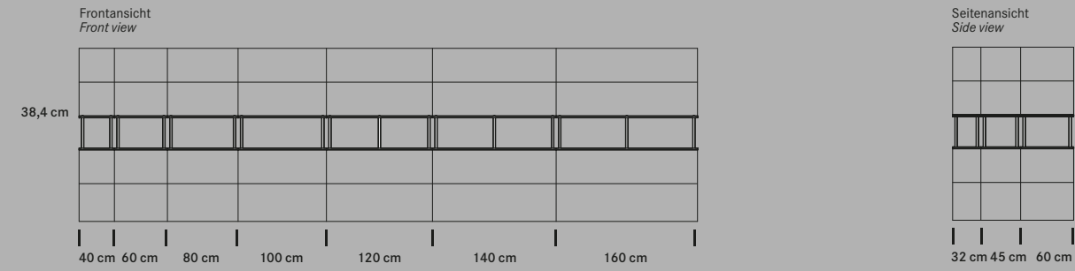
WINEA MAXX offene Mittelregale WINEA MAXX open intermediate shelves
