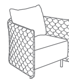
CLO-Q-1-LO Cloud armchair low quilted back metric (mm) W800 D750 H650 seat 400 imperial (in) W31.5 D29.5 H25.5 seat 15.5
