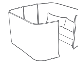
CLO-P-BOOTH-3 Cloud plain 3 seat booth metric (mm) W2100 D2200 H1300 seat 400 imperial (in) W82.5 D86.5 H51 seat 15.5
